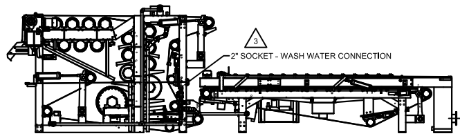
VIEW B-B
