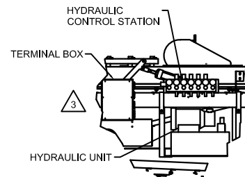
DETAIL B HYDRAULIC CONTROLS
