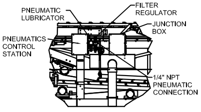
DETAIL C PNEUMATIC CONTROLS
