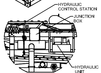
DETAIL C HYDRAULIC CONTROLS
