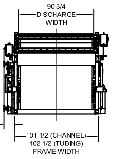
DETAIL C PNEUMATIC CONTROLS
