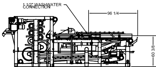
VIEW B-B
